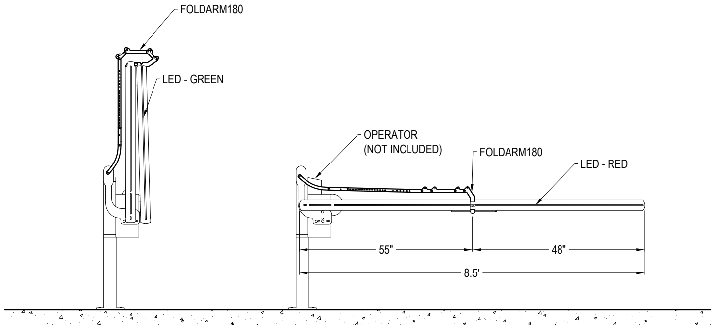
ELEVATION (GATE 180° ANGLE DOWN POSITION - FOLDARM180-44 SHOWN)
